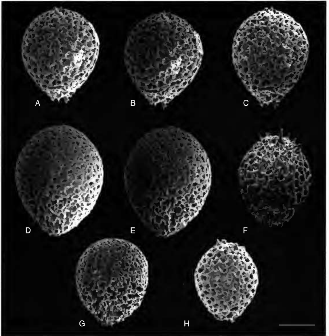
FIG. 8. — Glomeropyle aurora Aita, n. sp.; A-C, holotype (photo Nos 31101, 31102 & 31107); A, B, stereograph, C, lateral view; D, E, paratype (photo Nos 31123, 31125), stereograph; F, paratype (photo No. 31106); G, H, photo Nos 31109, 31110. Sample MAH-3.5, Unit 2, Mahinepua Peninsula, North Island, New Zealand. Scale bar: 100 \mu m.
